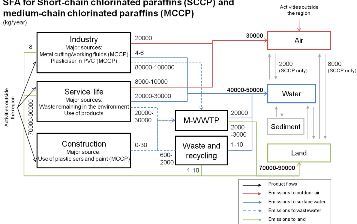
Figure 17: Simplified substance flow analysis (SFA) for short-chain chlorinated paraffins (SCCP) and medium-chain chlorinated paraffins (MCCP) in the Baltic Sea Region (c. 2008- c.2011). Numbers are rounded to one significant digit.
