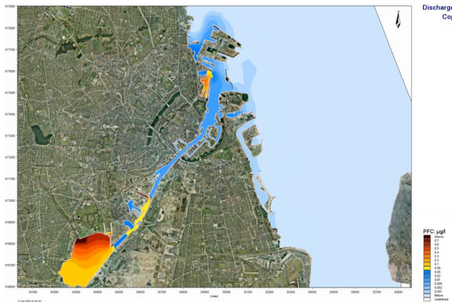
Figure 33: Hydrodynamic fate modelling of PFC in Copenhagen Harbour. The map illustrates the predicted situation after heavy rain in June 2009. This is a picture from the video animation, which can be viewed at www.cohiba-project.net .
